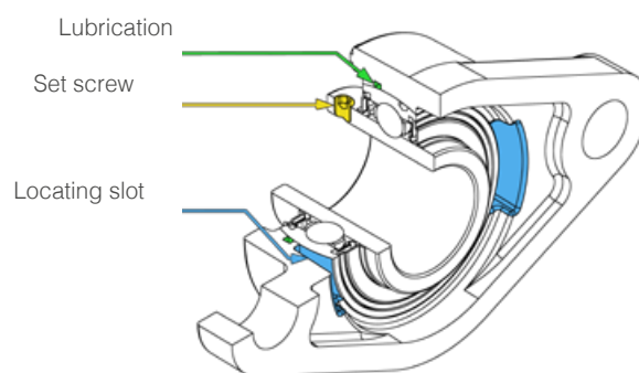
Bearing unit according to JIS B 1559
