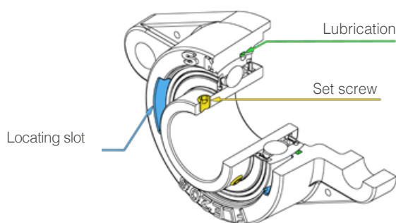
Bearing unit according to ISO 3228
