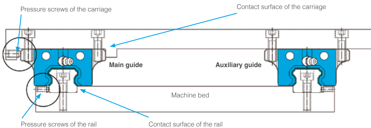
Figure 3.1 Installation of two parallel arranged Linear Guides
