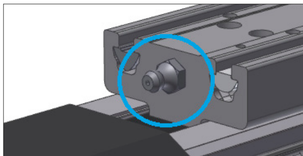
Figure 4.3 Lubrication points for AXE60Z, AXE80Z, AXE100Z
