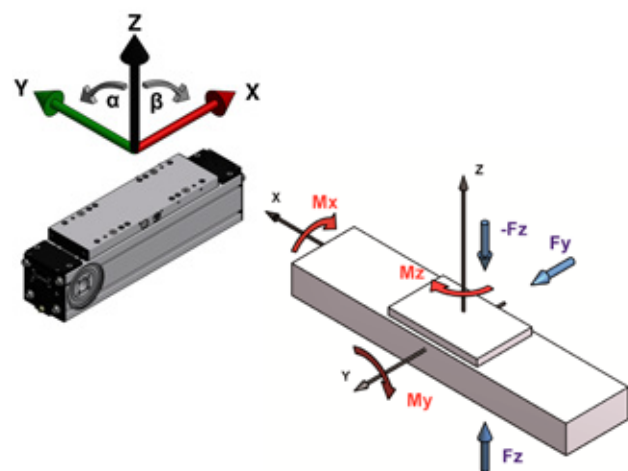
Figure 2.1 Coordinate system
