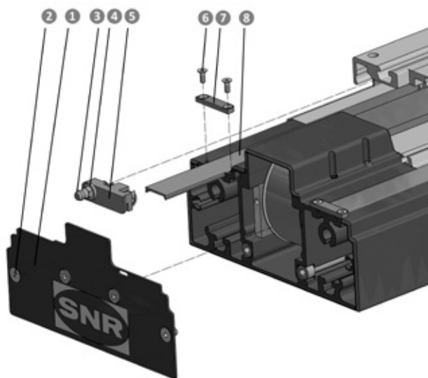
Figure 4.7 Cover strip replacement
