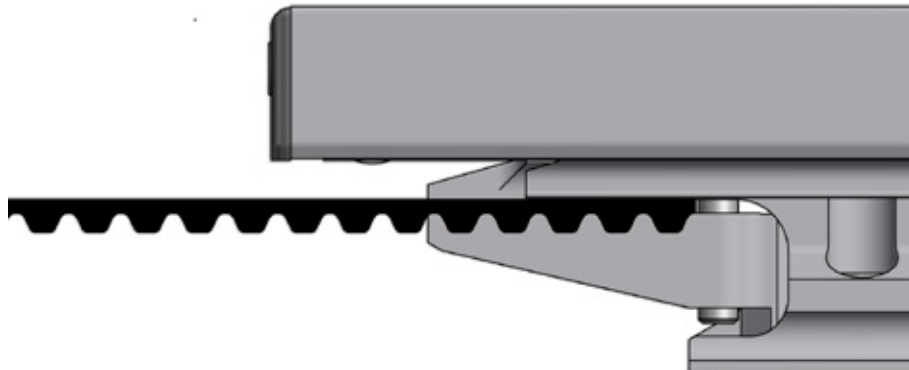
Figure 1.7 Toothed belt clamping
