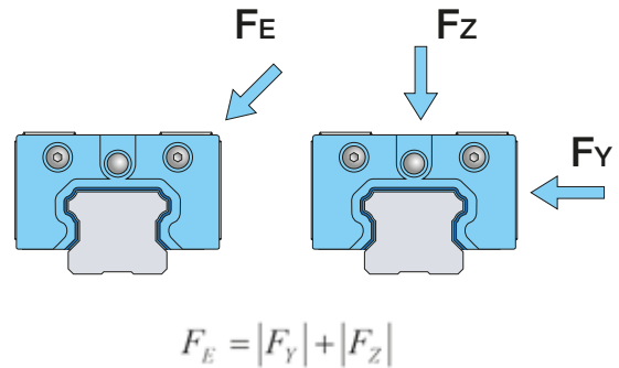
Figure 2.2 Equivalent load
