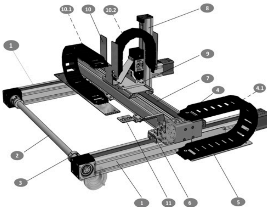
Figure 7.1 Standard Axis System
