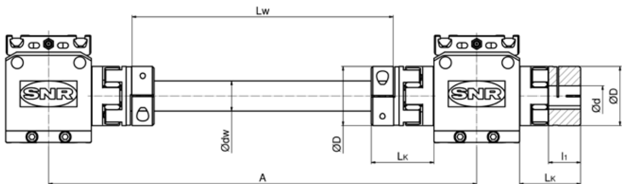
Figure 6.19 Dimension of couplings and connecting shaft
