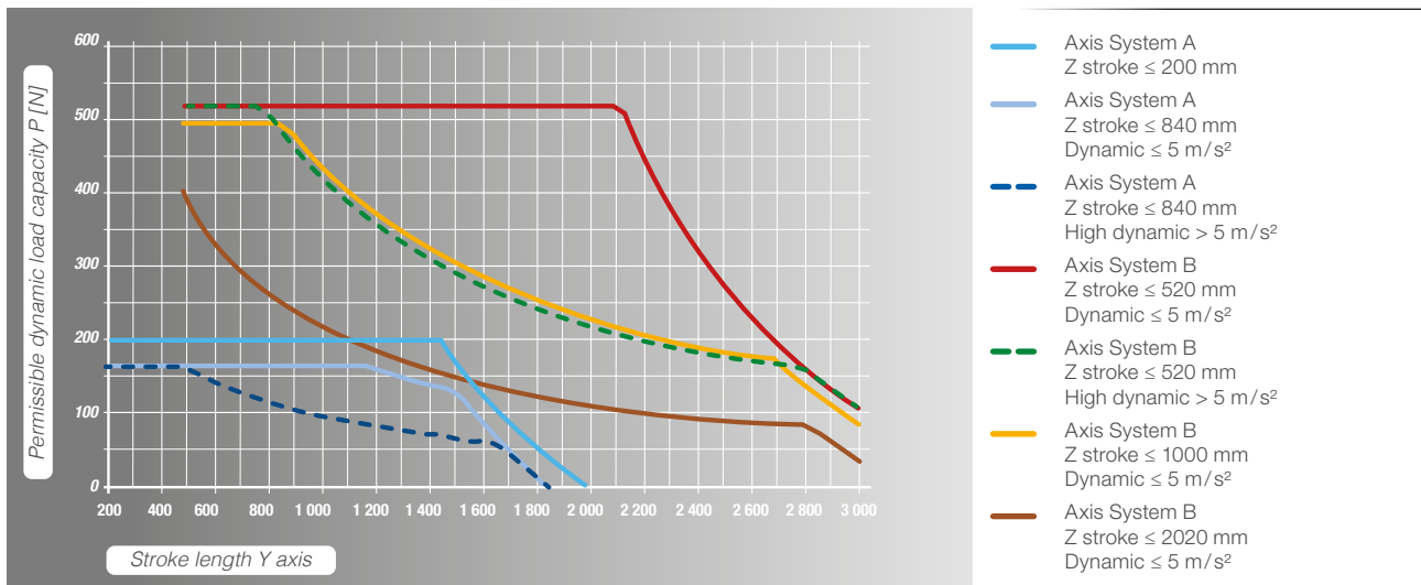
Figure 7.2 Dynamic load capacities of Standard Axis Stems
