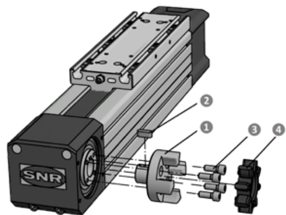
Figure 3.6 Force-fitted mounting of couplings on Linear Axis with toothed belt drive
