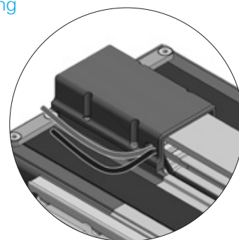
Figure 3.15 Cable guiding for inductive proximity switches AXE110Z
