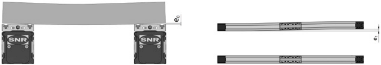
Figure 3.1 Tolerances of parallel linear axis
